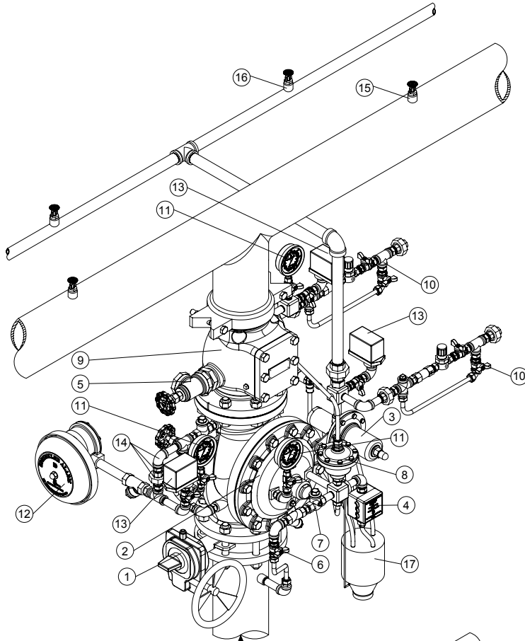
FRONT VIEW
