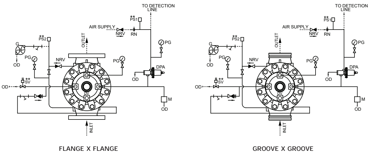
SCHEMATIC 4
