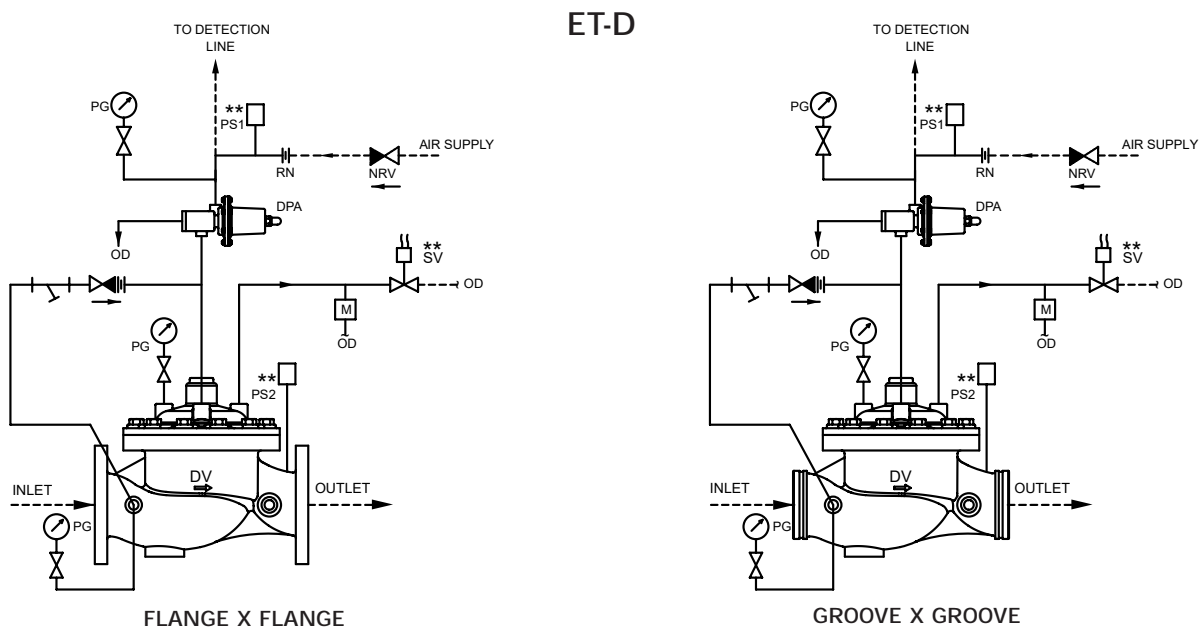
SCHEMATIC 10
