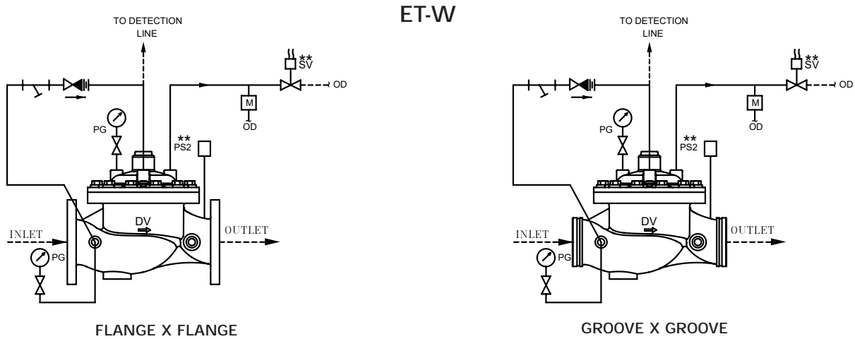
SCHEMATIC 9
