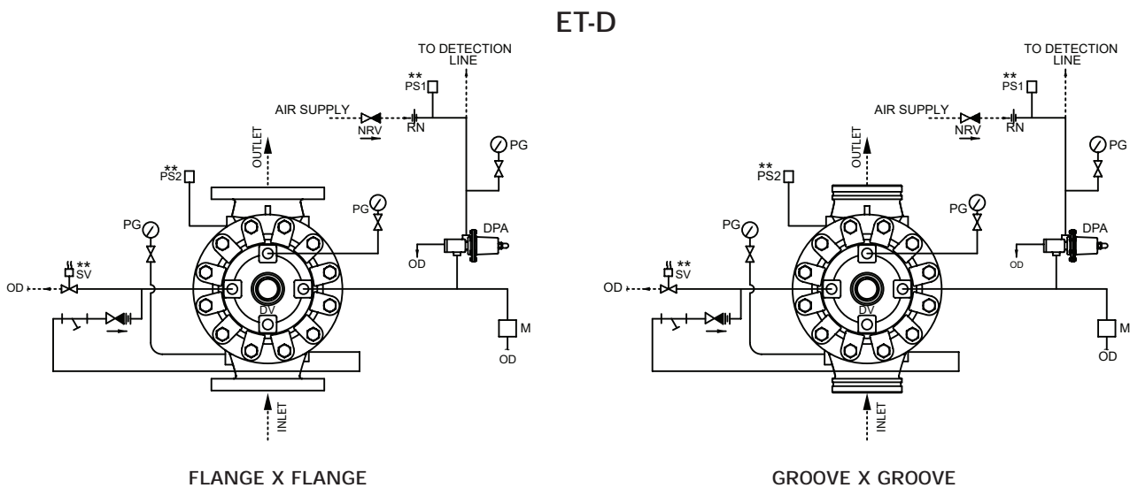
SCHEMATIC 2
