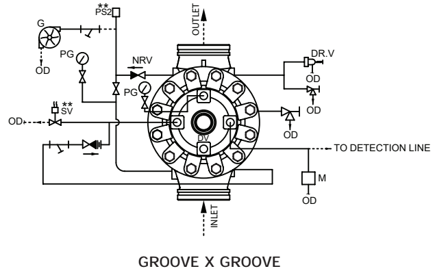
SCHEMATIC 7
