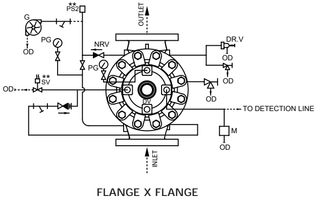
SCHEMATIC 7
