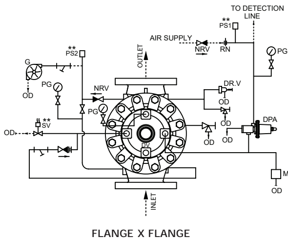
SCHEMATIC 8
